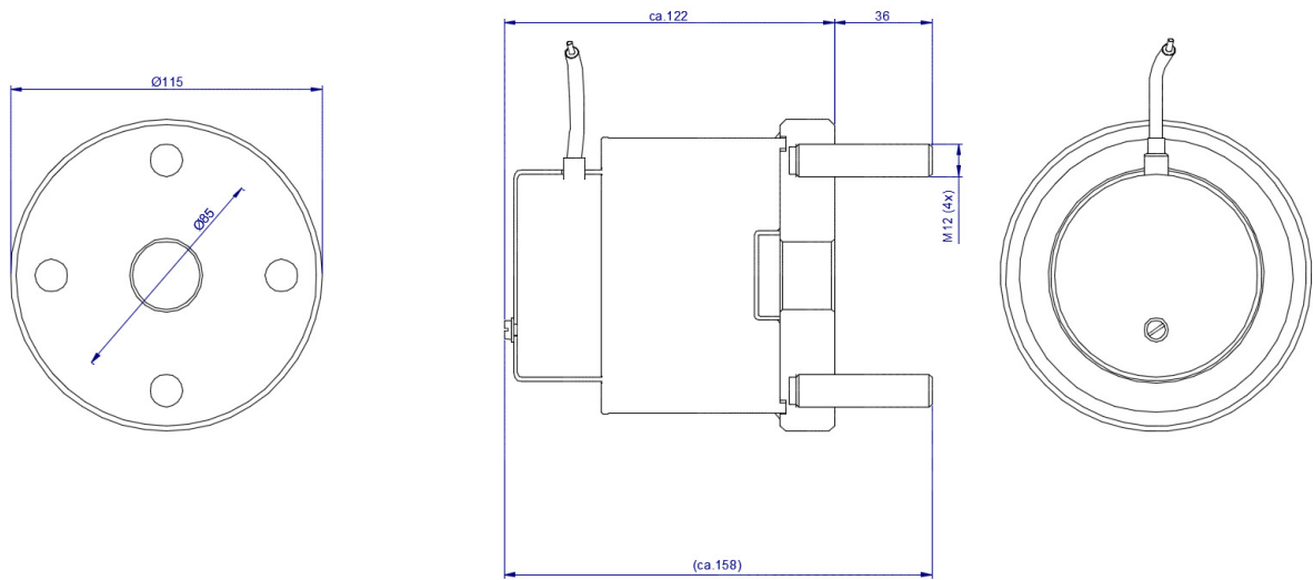
Dimensions (mm)
